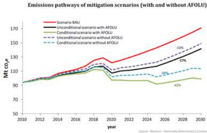
Figure 1 Emissions pathways of mitigation scenarios (with and without AFOLU)
